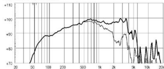
FREQUENCY RESPONSE CURVE
