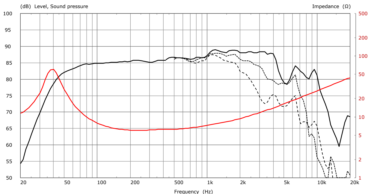
20-400Hz Frequency Response on 18 Lt @ 40 Hz Vented Box @ 1W, 1m 400-20000Hz Frequency Response on IEC Baffle (DIN 45575) @ 25cm, normalized to SPL 1W,1m Dotted line off-axis Frequency response at 30°,60° - Free Air Impedance Measurement in Anechoic Chamber
